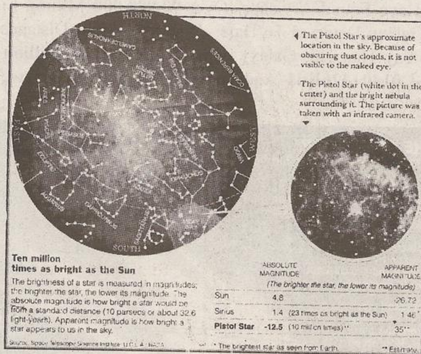
Figure 14 Pistol Star
