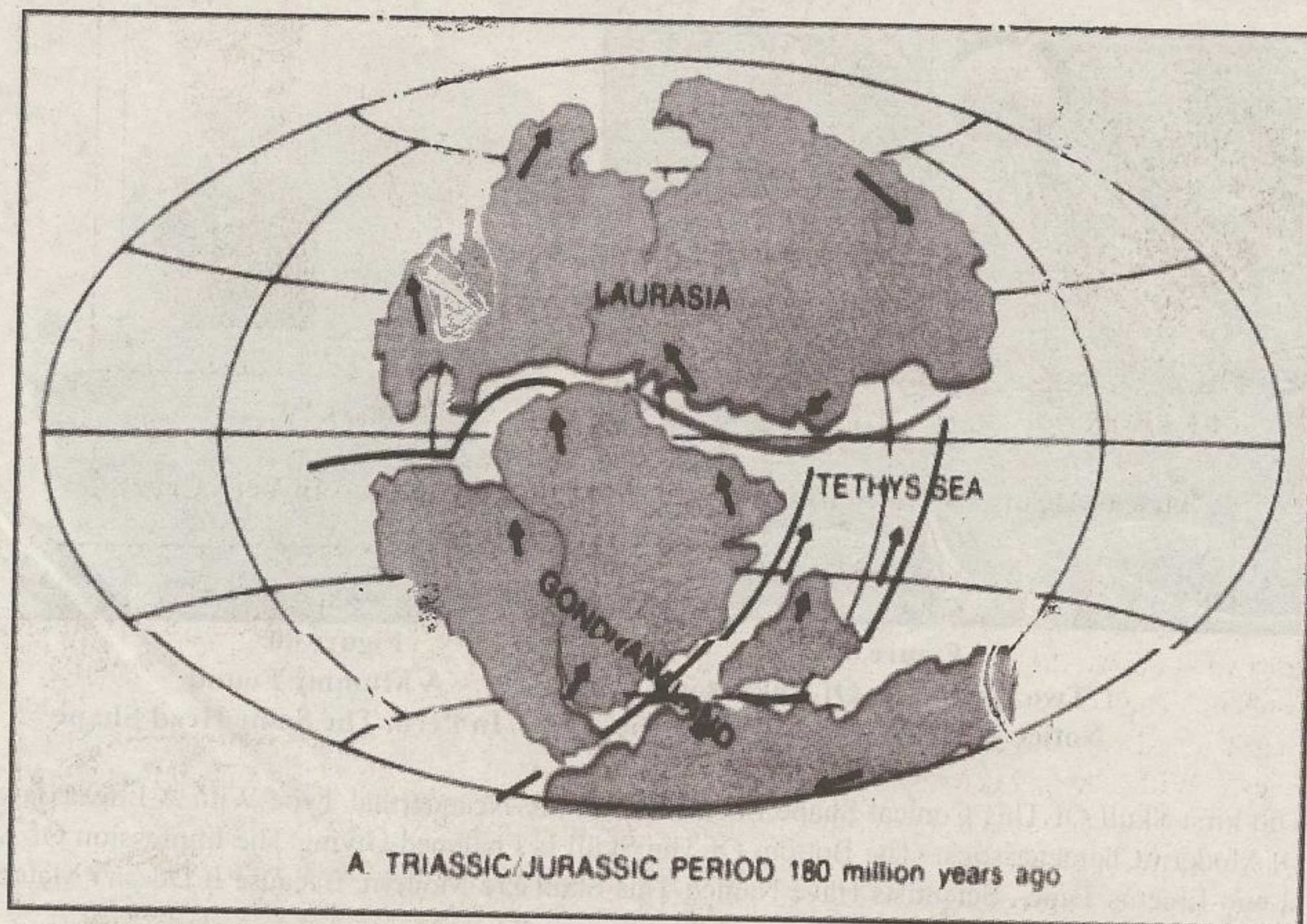
Diagram 23 The Land Mass Before Continental Drift
