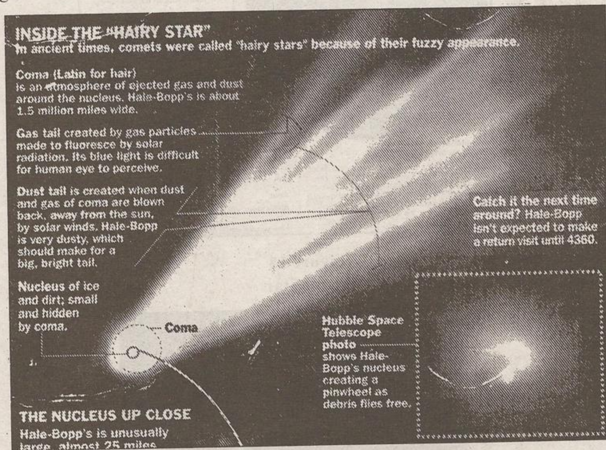
Figure 13 Hale-Bopp/Nibiru
