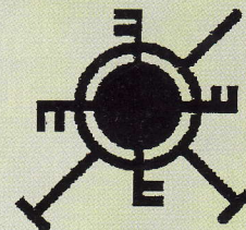
Light around comet.
