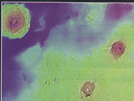
Martian volcanoes, such as these, may have been responsible for the meteorite containing the ancient fossil found in Antarctica by NASA.
