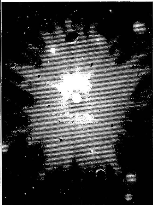
Diagram 16 Picture Of The Big Bang Theory.
