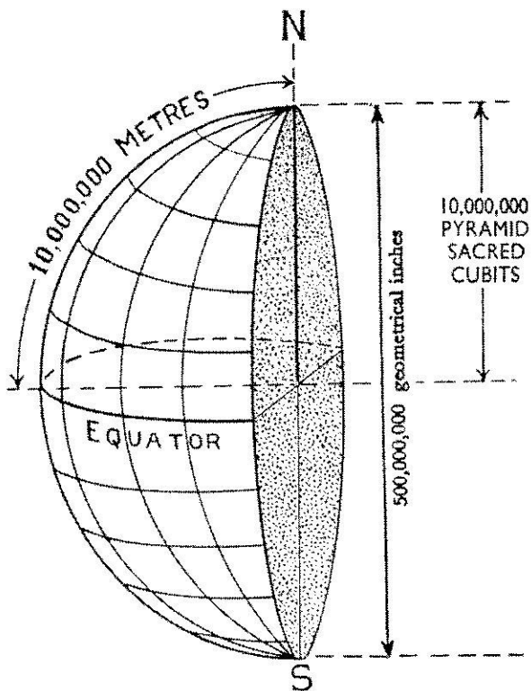
Diagram 44 The Earth's Polar Radius Measurements.
