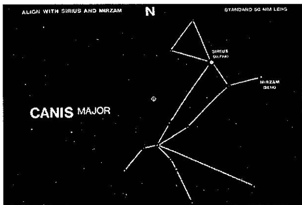
Diagram 25 Orion Constellation With The Sirius Star Constellation To Its Left.
