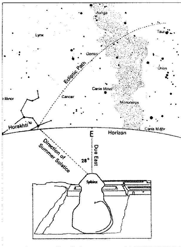
Diagram 39 Epoch Of The Pyramid Age: The Rising Of Leo At The Summer Solstice.
