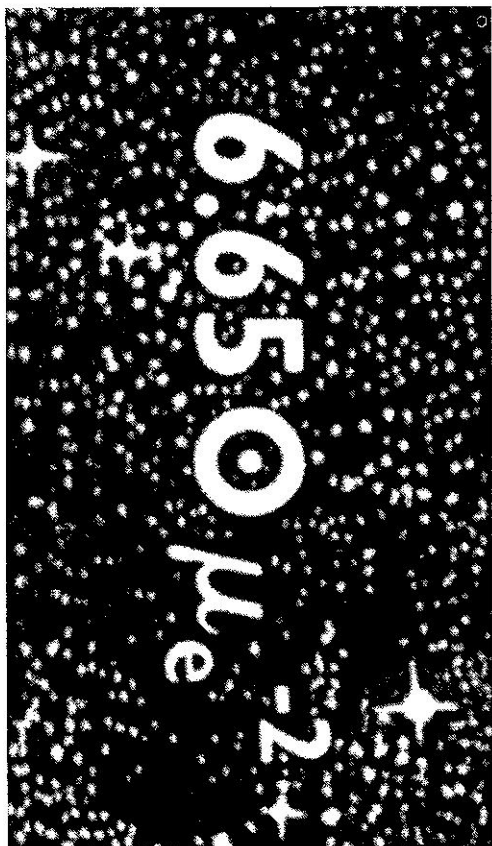
Figure 116 A White Dwarf
