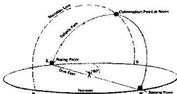
17. The trajectory of the sun on the equinox.
