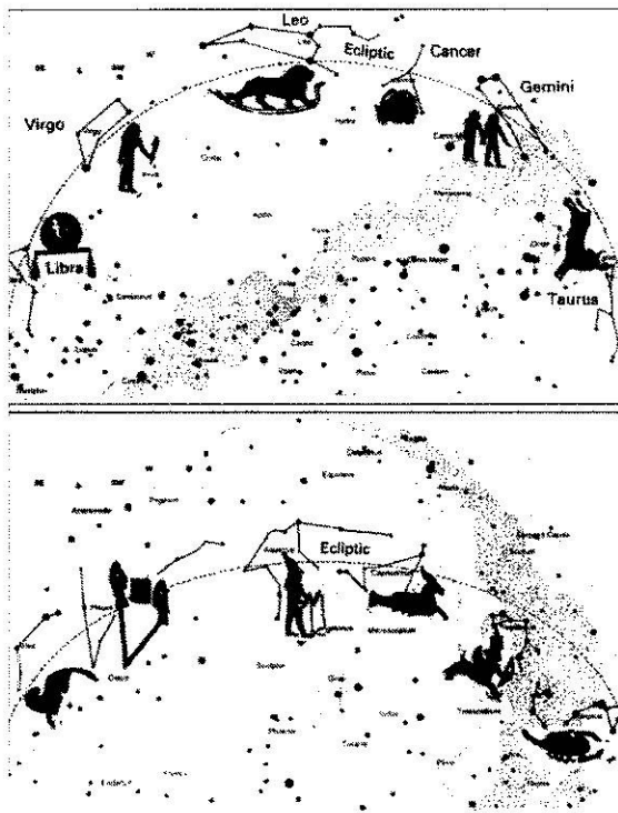
Diagram 12 The Path Of The Sun (The Ecliptic) Passing Through The Twelve Zodiacal Constellations As They Are Depicted In The Famous Denderah Zodiac From Upper Egypt.
