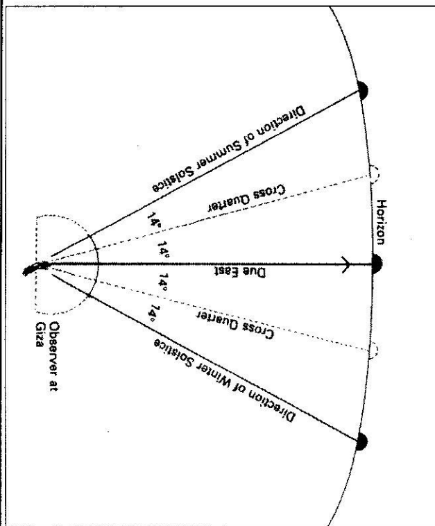
Diagram 21 The Course Of The Sun Throughout The Year As Viewed From The Latitude Of Giza.
