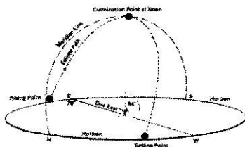
16. The trajectory of the sun on the summer solstice, with its culmination point (highest altitude) being attained at meridian transit.
